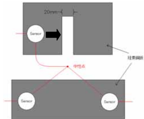
Fig.2 Target Silicon Steel and Moving Direction of the Sensor
