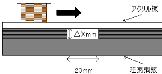
Fig.6 Schematic Diagram for the Hollow Sensing
