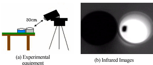
Fig.2 Ice Melting by Boiled Water
