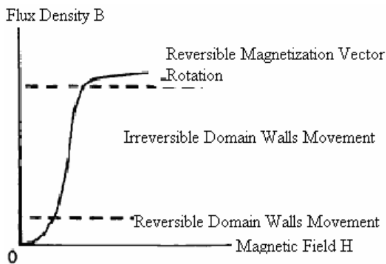
(b) Typical magnetization curve of ferromagnetic materials.
