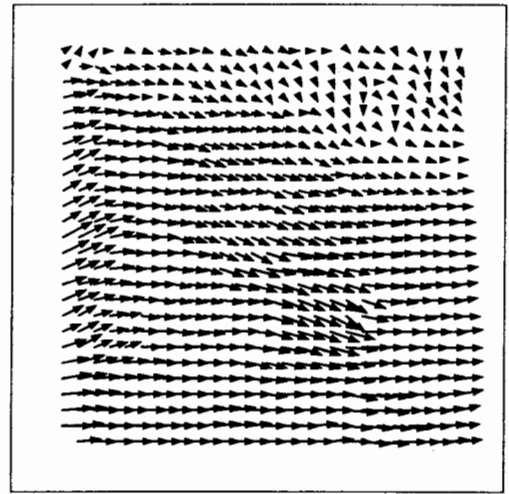
Fig.4 Velocity vector field obtained from the cross-correlation of compressed PIV image pair
